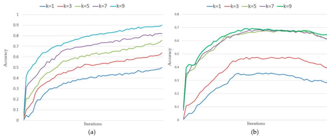
Figure 8. Indoor-WhereNext frame location prediction accuracy: (a) accuracy of location prediction on training dataset and (b) accuracy of location prediction on test dataset.
